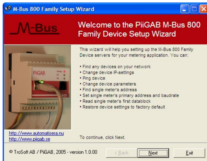
Figure 4-1. Welcome Screen
