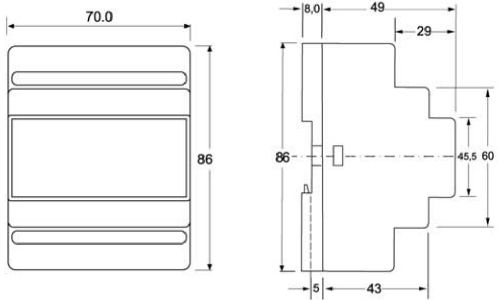
Figure 2-1. Cabinet
