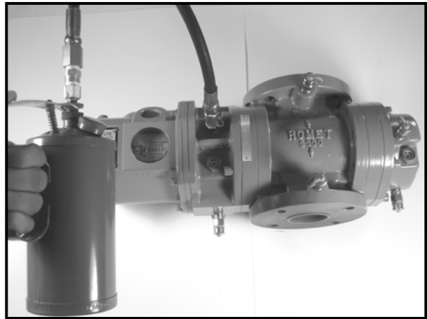
Model 1600 Oiler
