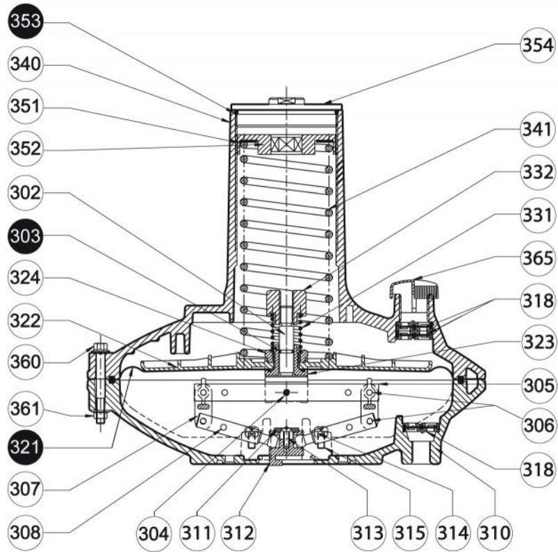
fig. 23 Standard head
