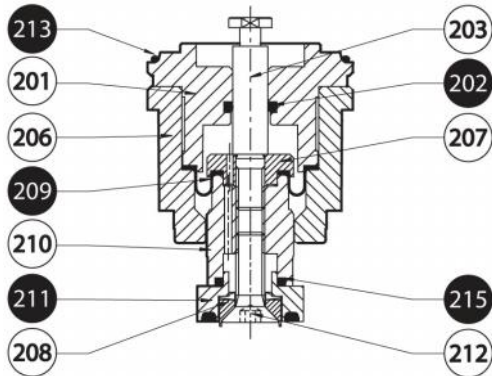
fig. 25a (Standard version DN 25 e 32)
