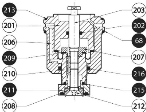
fig. 26a (Monitor version DN 25 e 32)
