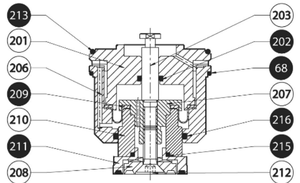
fig. 26b (Monitor version DN 40 e 50)
