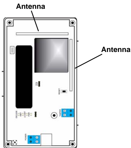
Figure 3 High power repeater antenna orientation
