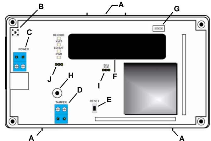
Figure 2 High power repeater internal components
