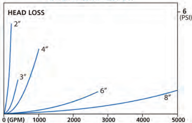
HEAD LOSS CHART
