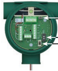
Separate USB Communication Channel 3-Way Switch for the 4-20 mA Output On/Off Power Switch
